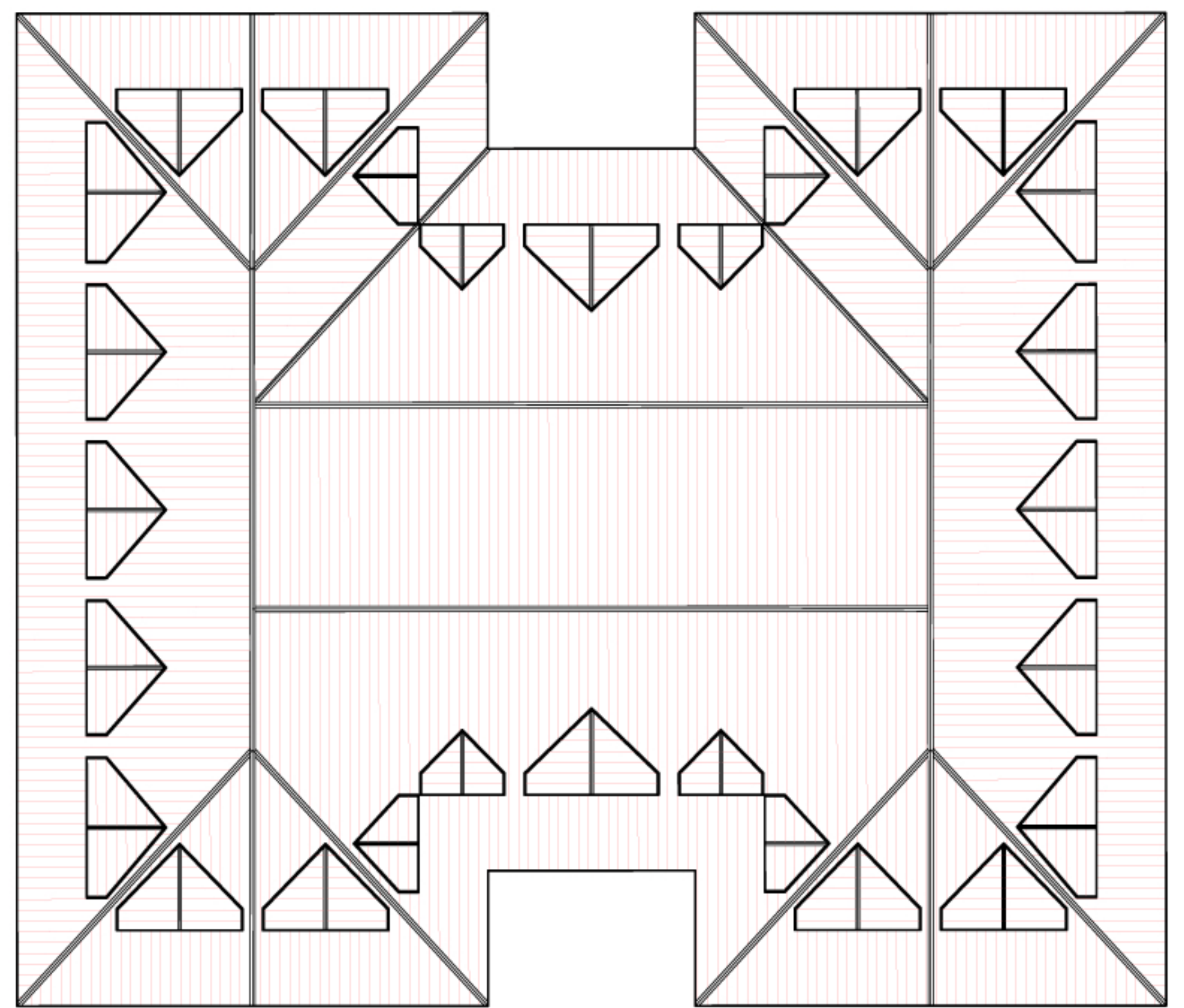
ROOF LEVEL ARCHITECTURAL FLOOR PLAN
