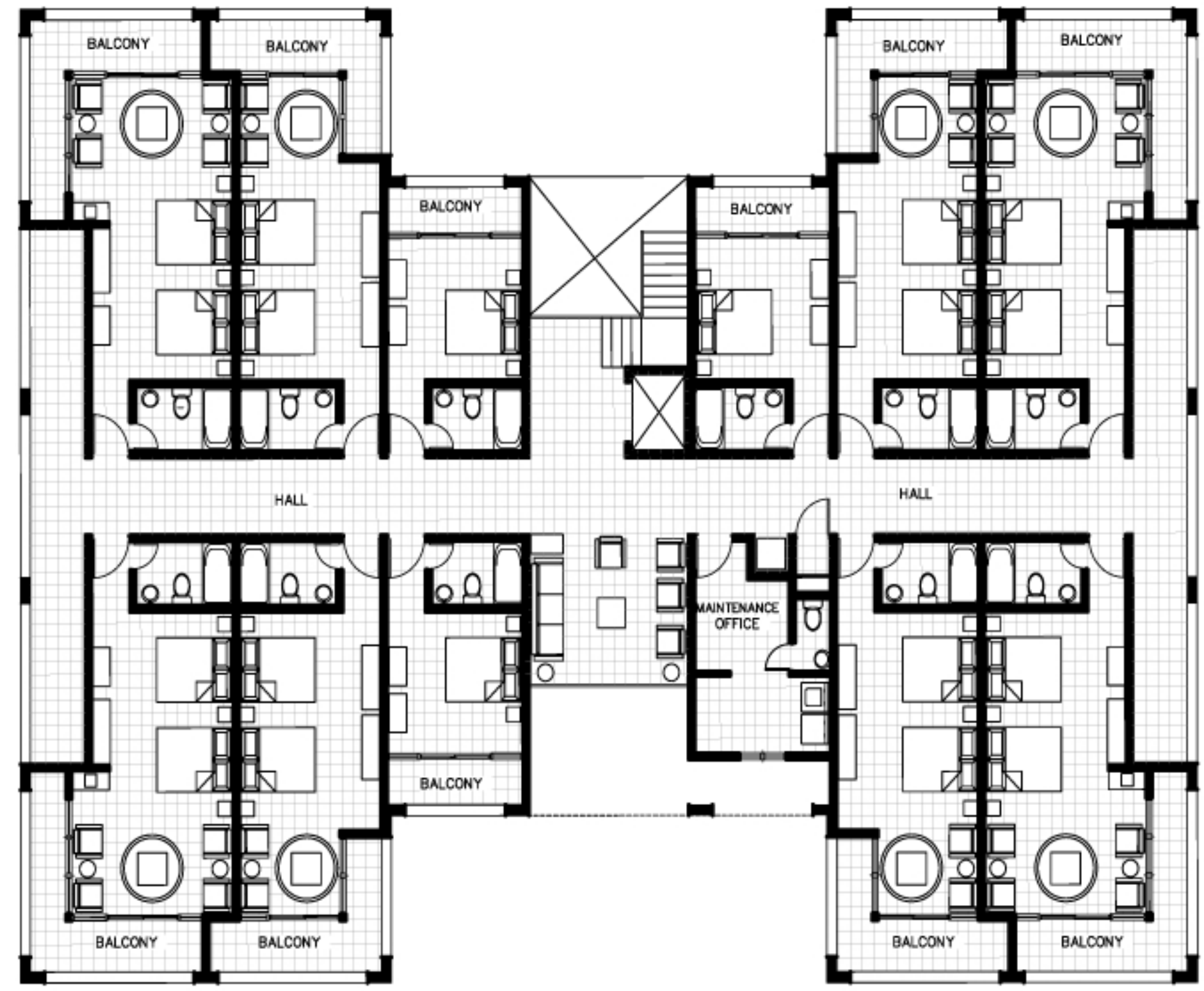
SECOND AND THIRD LEVELS ARCHITECTURAL FLOOR PLAN
